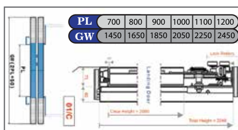
Central two panels landing door
