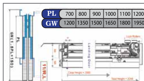
Telescopic two panels landing door
