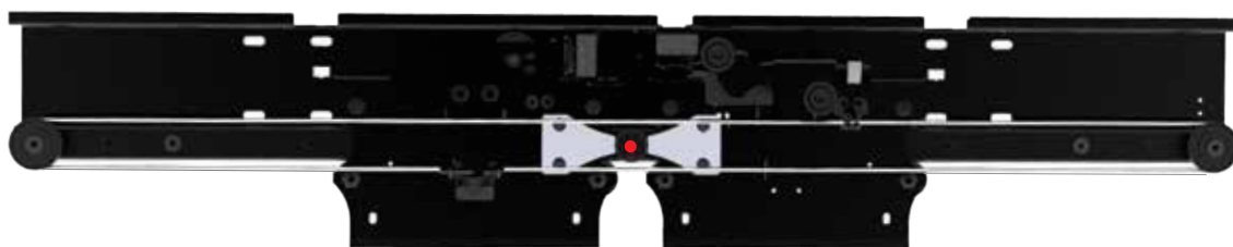
Two panel central landing door mechanism
